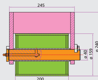
Drsnik ABROLL 200 mm
