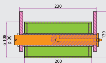
Drsnik AVIE 200 mm
